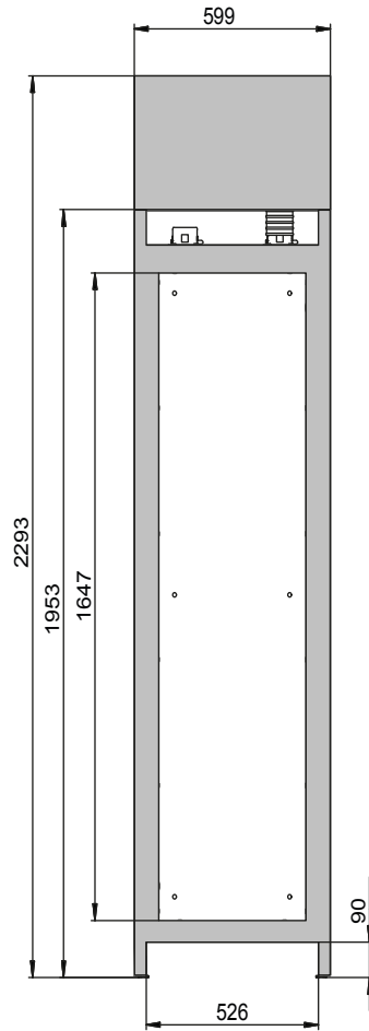
Front view
